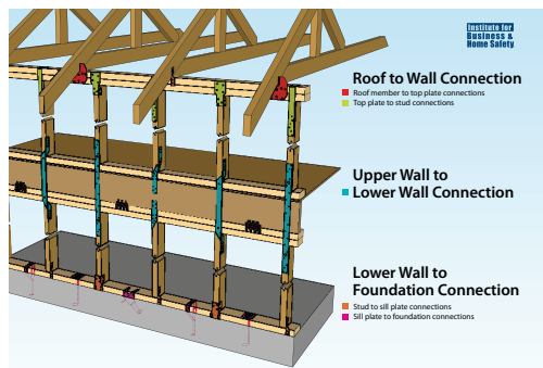
Continuous Load Path To Resist Uplift Forces
