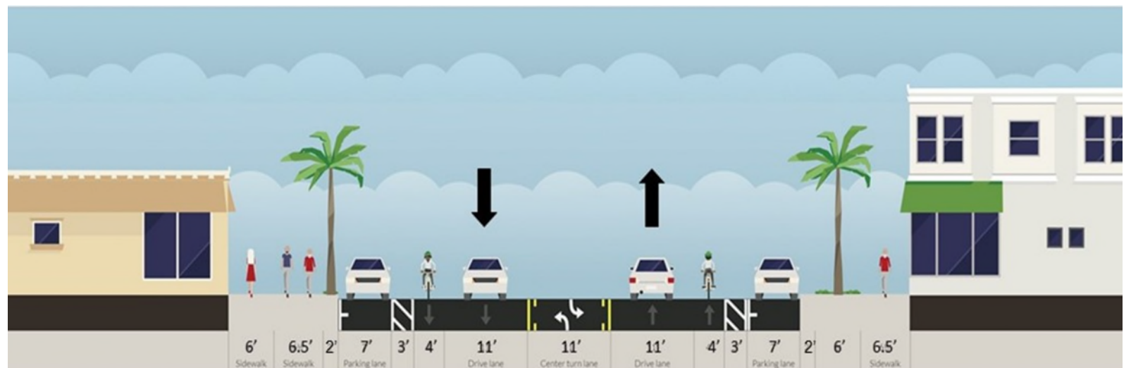
SR 811 Typical Section from Middle River Bridge—NE 26th Street
