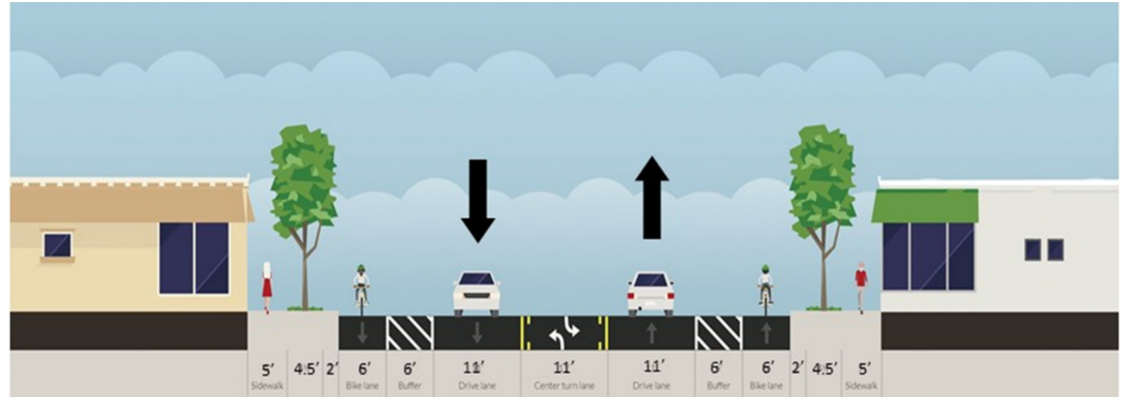
SR 811 Typical Section from Sunrise—Middle River Bridge
