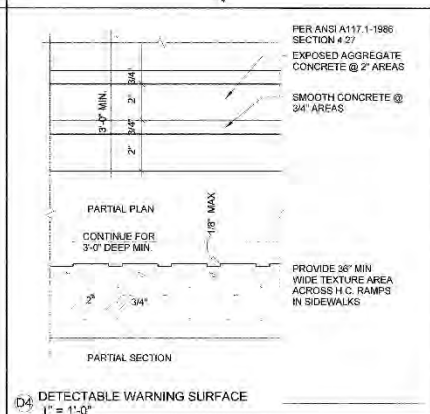
D4 DETECTABLE WARNING SURFACE 1" = 1'-0"
