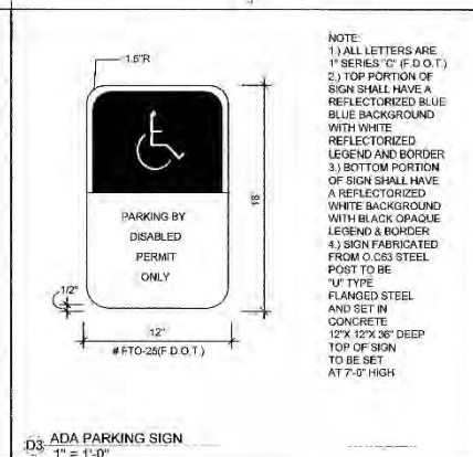
D3 ADA PARKING SIGN 1" = 1'-0"
