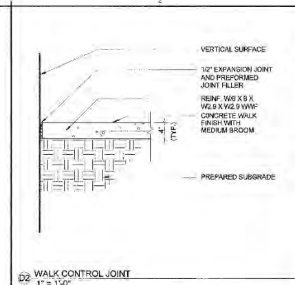
D2 WALK CONTROL JOINT 1" = 1'-0"
